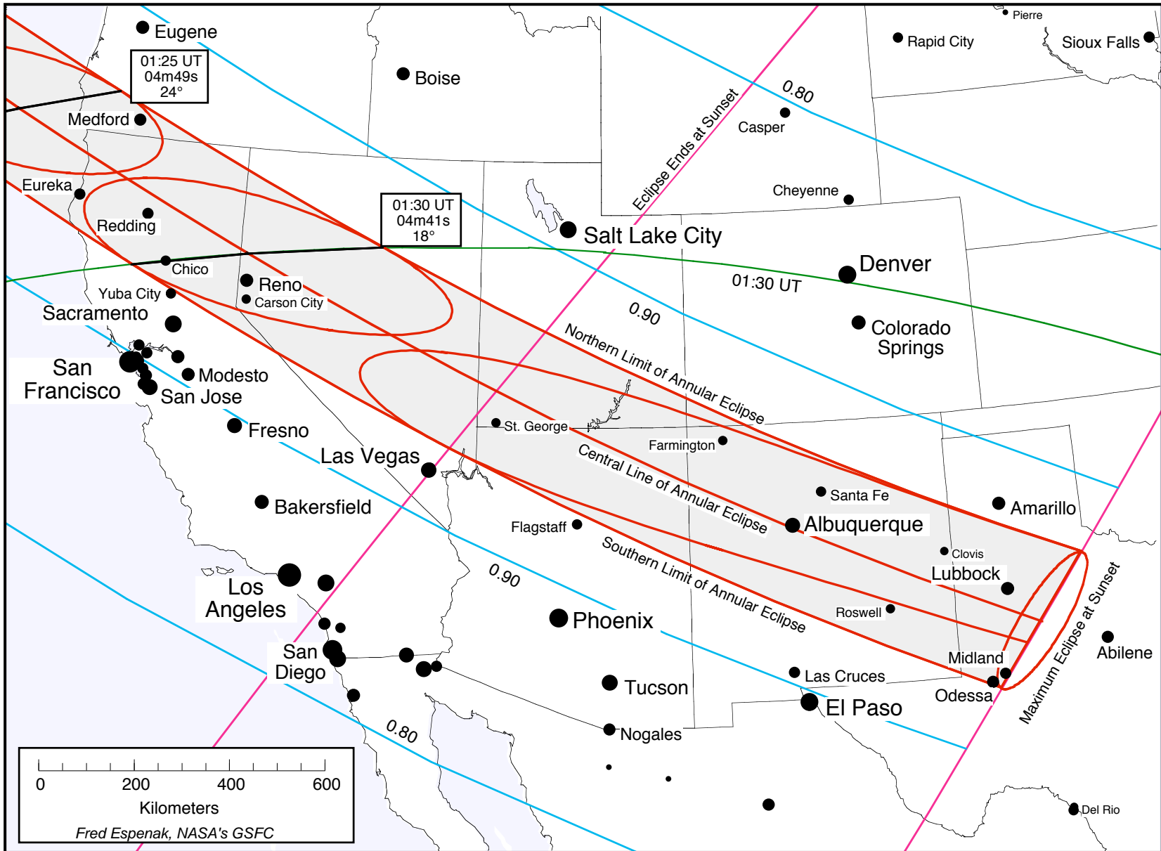
FIGURE 2 Annular Solar Eclipse of 2012 May 20
